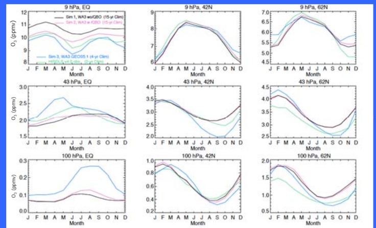
Figure 3: Comparisons of O 3 (ppmv) at the Equator, 42° N, and 62° N at three pressure levels (9 hPa, 43 hPa, and 100 hPa). Two 15-year climatologies (1993-2007) were created for simulation 1 and 2 (black and solid red lines respectively). A 4-year climatology was created for Simulation 3 (blue line). A two year climatology was created using the HIRDLS data for years 2006 and 2007 (green line).
