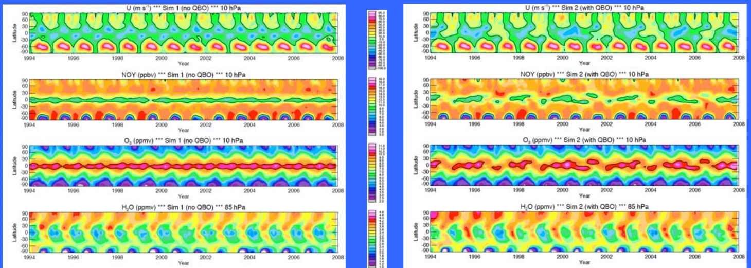
Figure 1: Latitude-time cross section of U, NO y , O 3 , and H 2 O. Simulation 1 (without QBO) on the left; Simulation 2 (with a QBO forcing) on the right.
